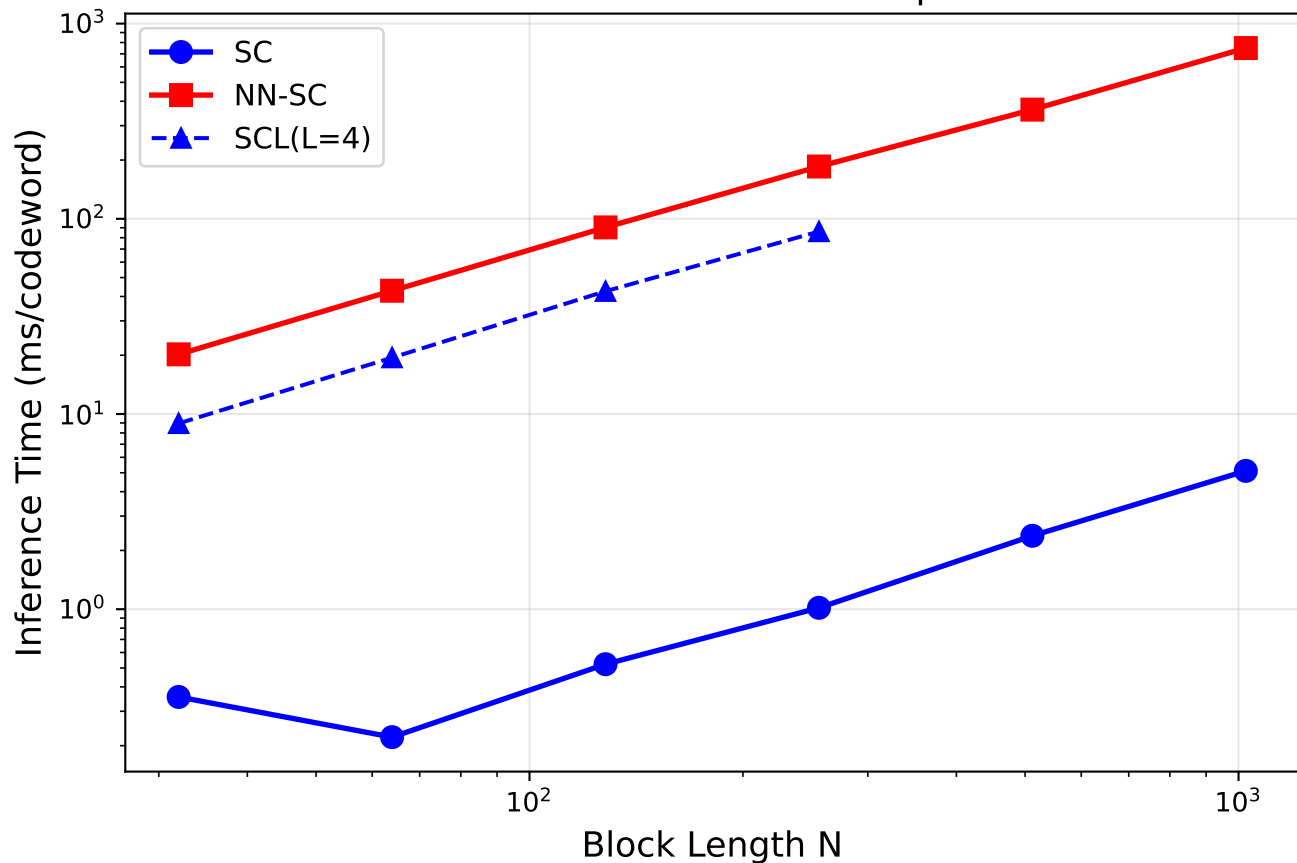
Decoder Inference Time Comparison
