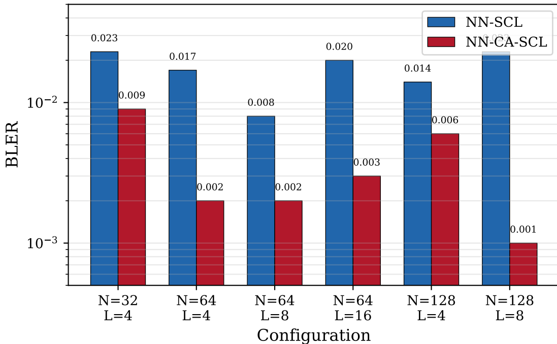
CRC-Aided Neural SCL: GMAC Class B, SNR=6dB
