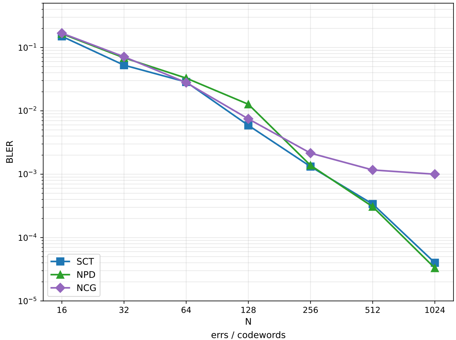
ISI-MAC corner-rate BLER vs N h=0.3, SNR=6 dB
