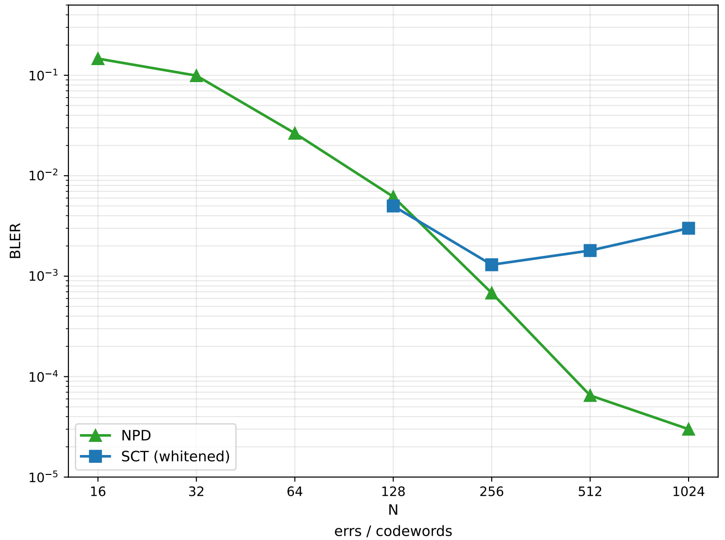
MA-AGN corner-rate BLER vs N \alpha=0.5 , SNR=6 dB
