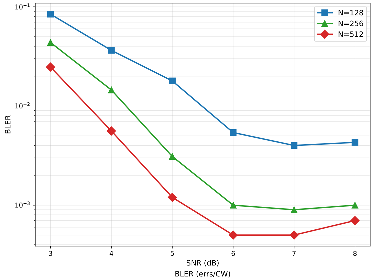
ISI-MAC SCT BLER vs SNR h=0.3, Class C corner-rate
