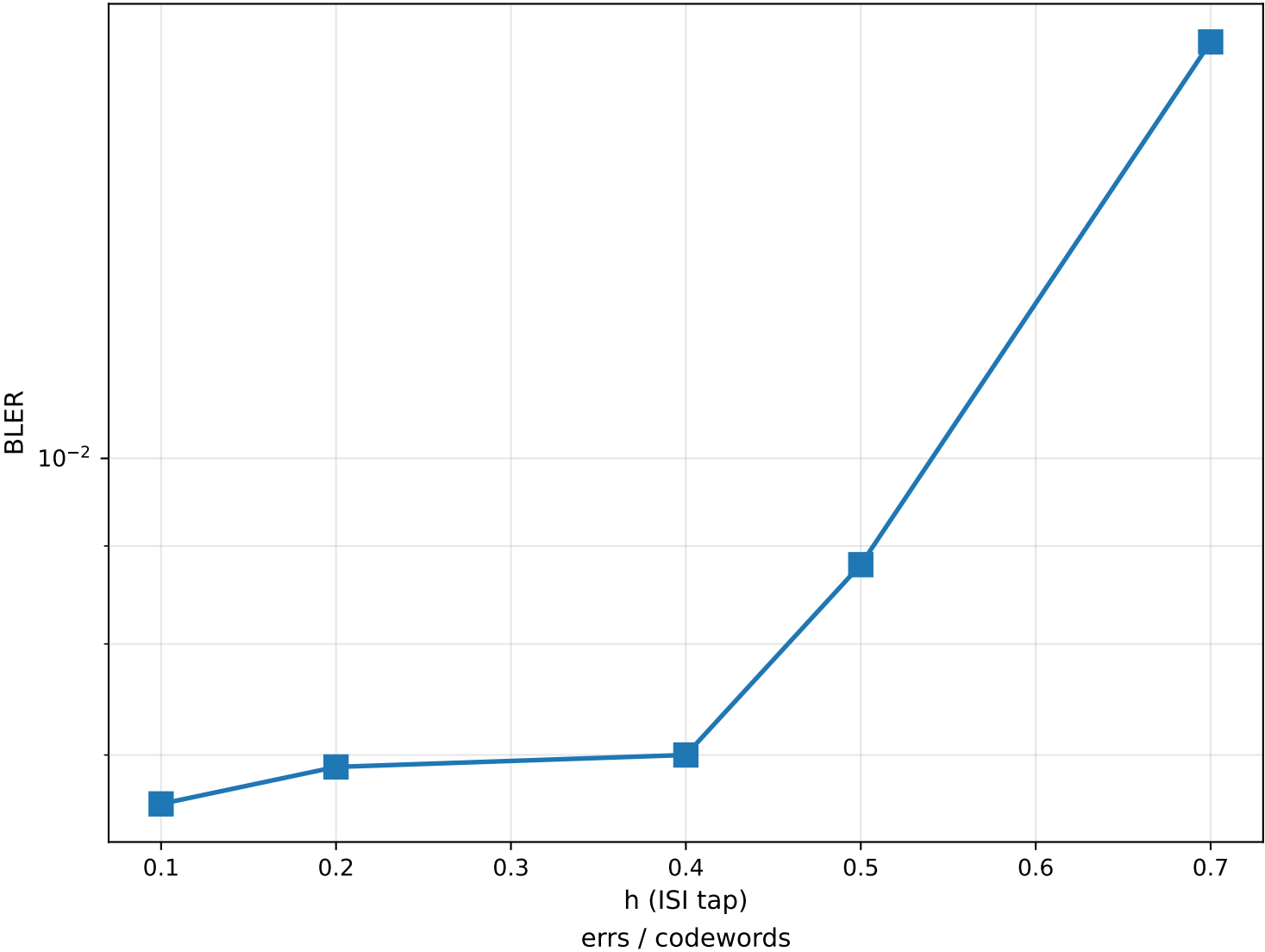
ISI-MAC SCT BLER vs h N=128, SNR=6 dB, corner-rate
