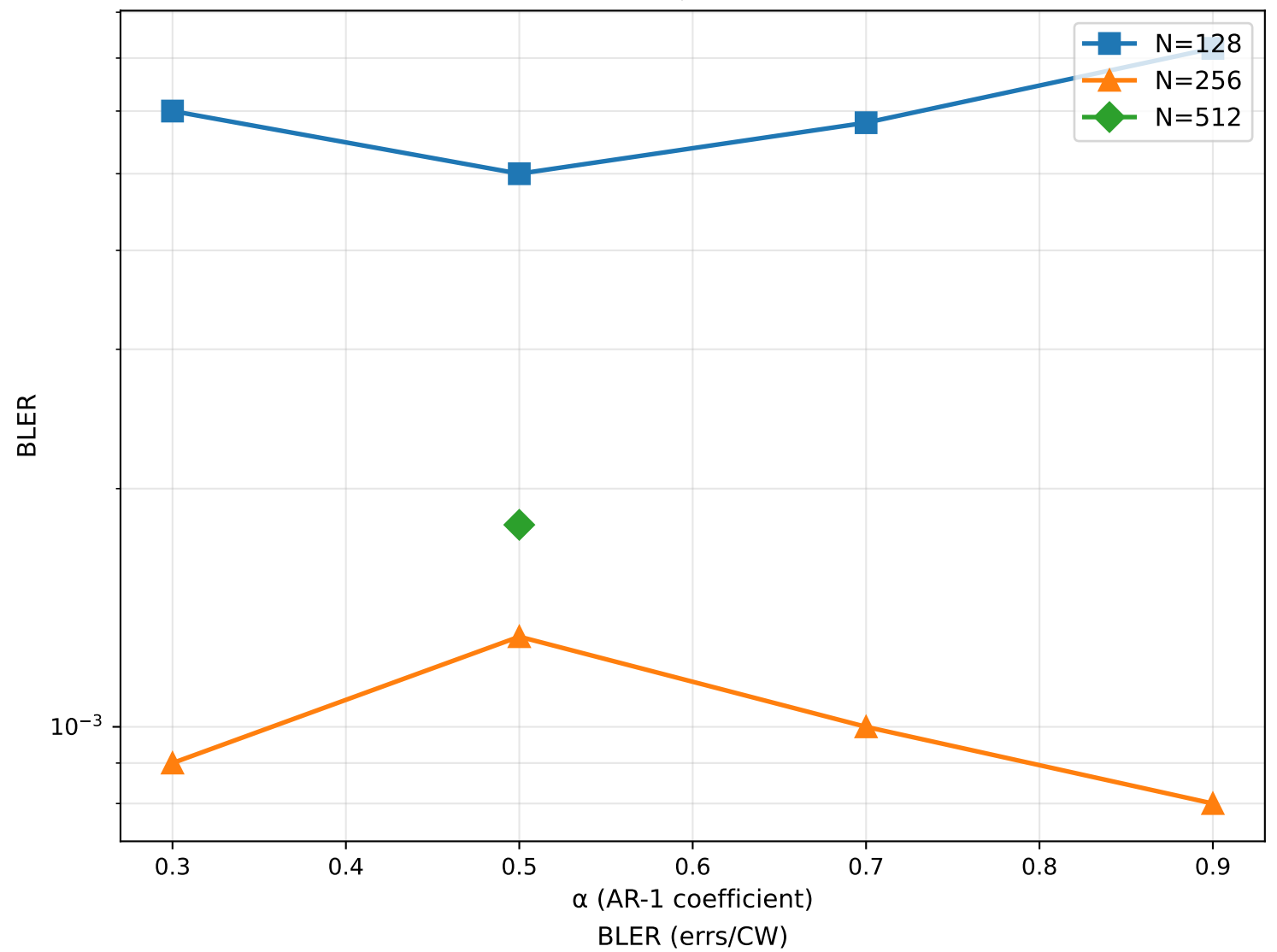
MA-AGN SCT BLER vs \alpha SNR=6 dB, corner-rate
