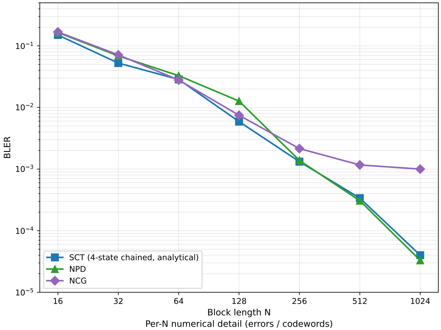
ISI-MAC corner-rate: SCT vs NPD vs NCG h=0.3 , SNR=6 dB, Class C
