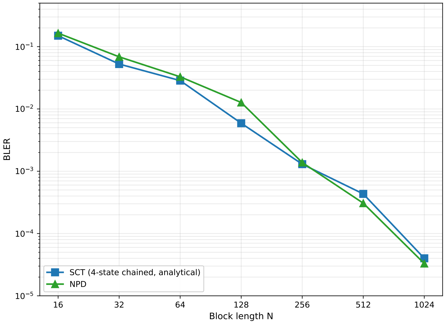
ISI-MAC corner-rate: analytical SCT vs NPD h=0.3 , SNR=6 dB, Class C
