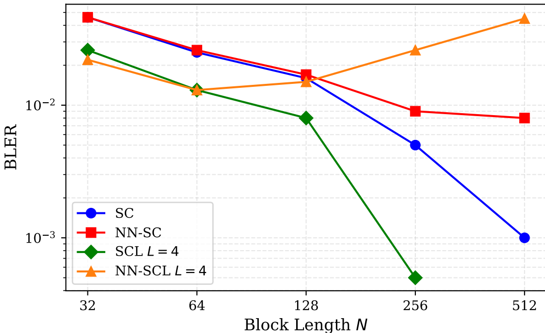
GMAC Class B (SNR = 6 dB): BLER vs Block Length
