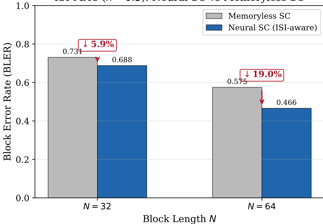
ISI-MAC ( h = 0.3 ): Neural SC vs Memoryless SC
