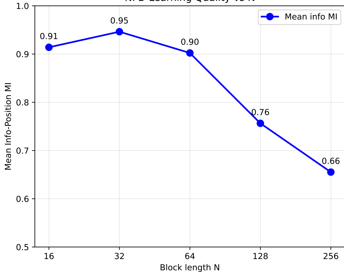
NPD Learning Quality vs N
