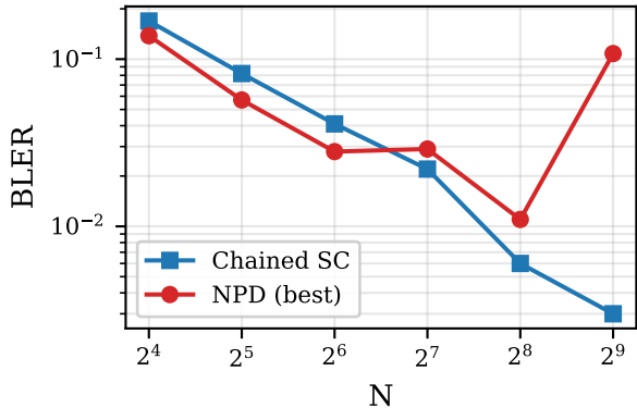
ISI-MAC (Chained SC vs Best NPD)
