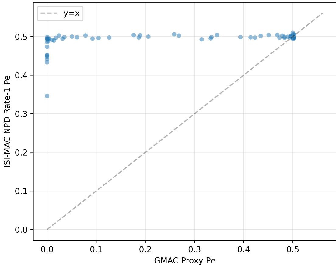
ISI vs GMAC Error Rate (N=64)
