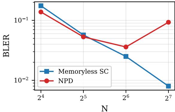
MA-AGN \alpha = 0.3
