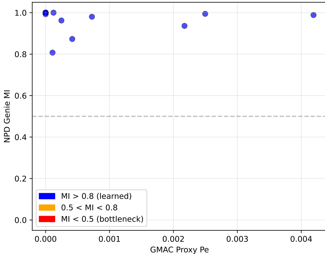
N=64: Info Position MI vs GMAC Proxy Quality
