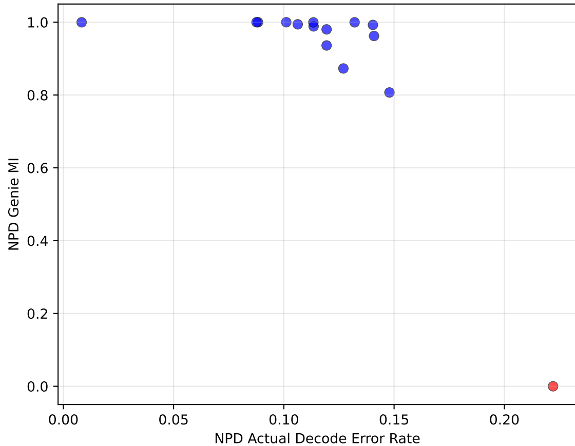
N=64: MI vs Decode Error (Info Positions)
