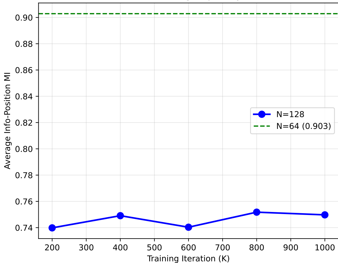
MI Learning Trajectory
