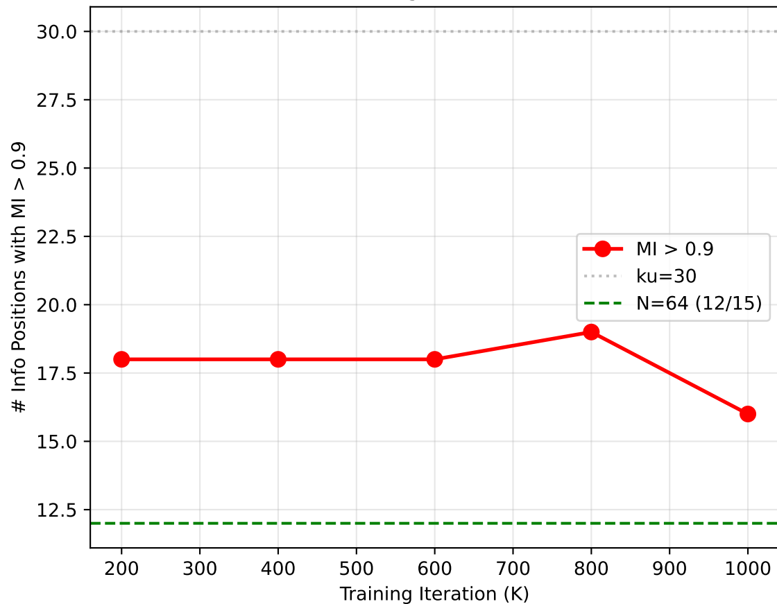
Polarization Progress (out of ku=30 )
