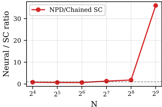
ISI-MAC: NPD/SC Ratio vs N
