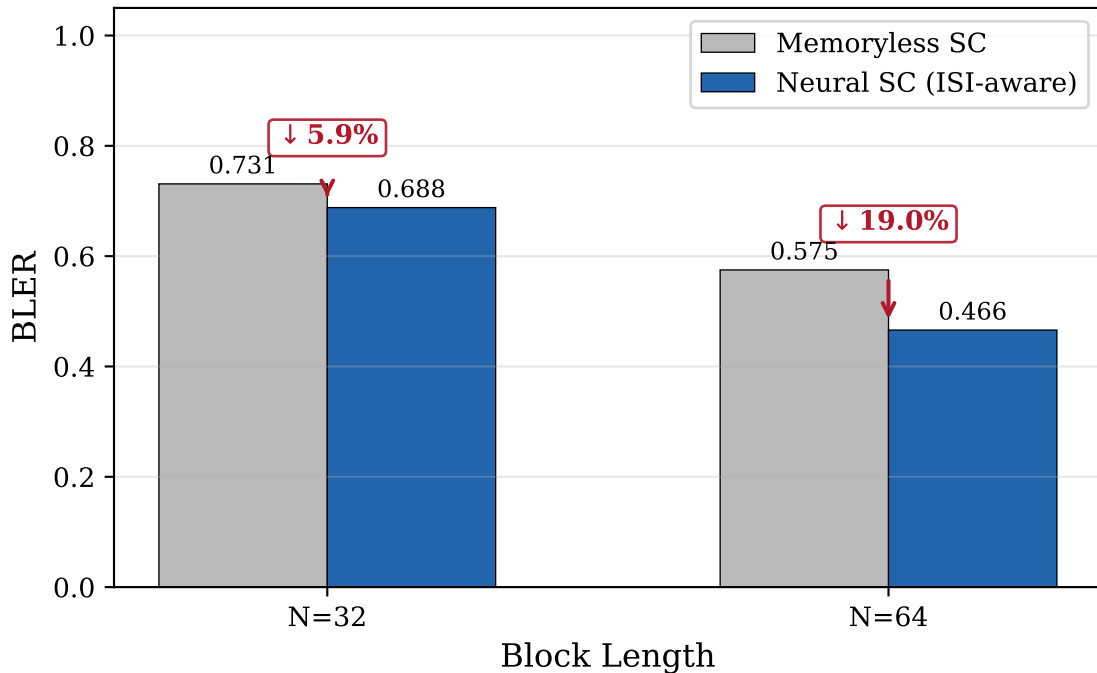
ISI-MAC ( h = 0.3 ): Neural vs Memoryless SC
