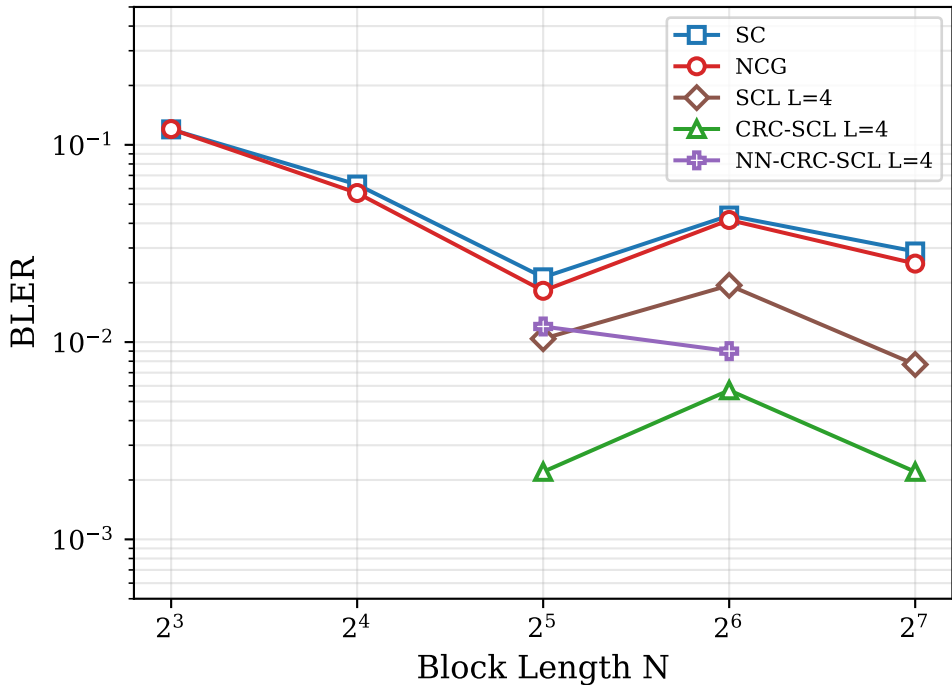
ABNMAC Class B: BLER vs N
