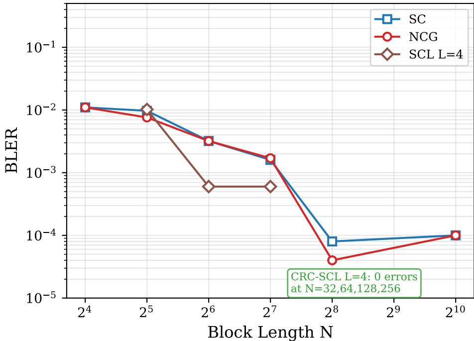
BEMAC Class B: BLER vs N
