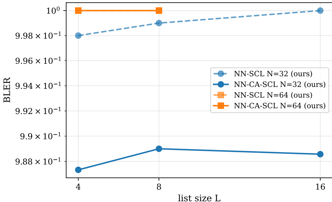
CRC-aided Neural SCL — ABN-MAC, Class B
