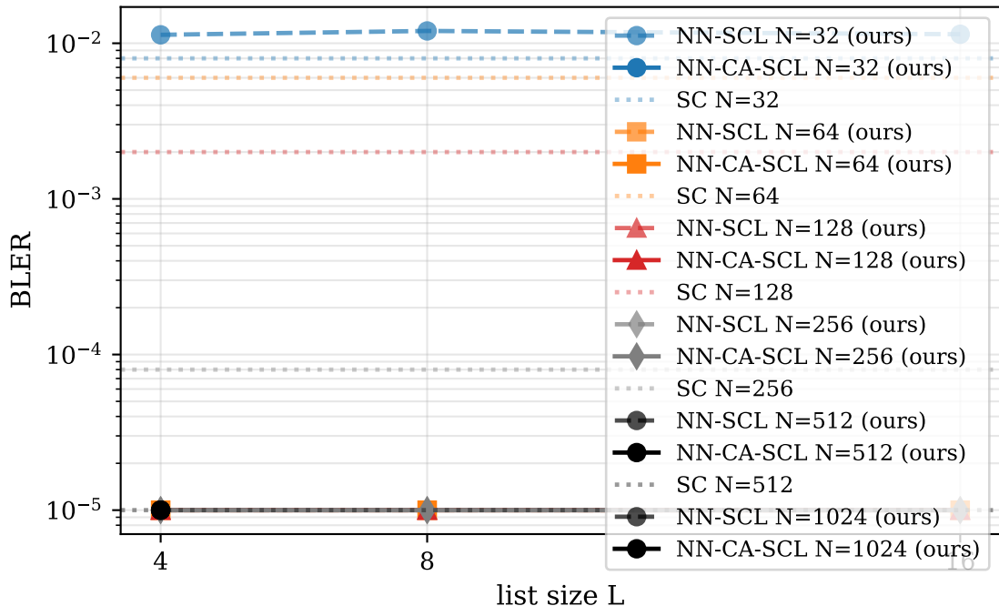
CRC-aided Neural SCL — BE-MAC, Class B
