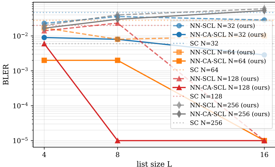
CRC-aided Neural SCL — Gaussian MAC (6 dB), Class B
