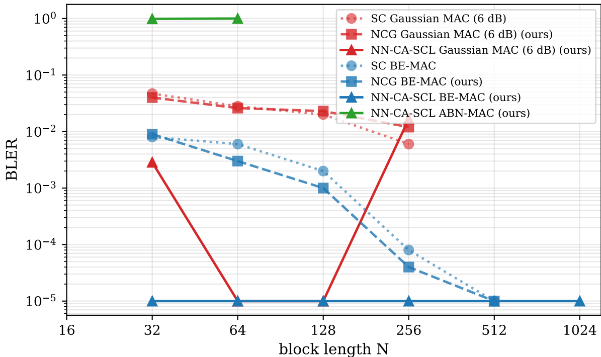
CRC-aided Neural SCL across channels — headline
