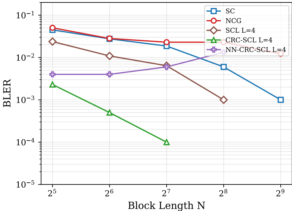
GMAC Class B (6 dB): BLER vs N
