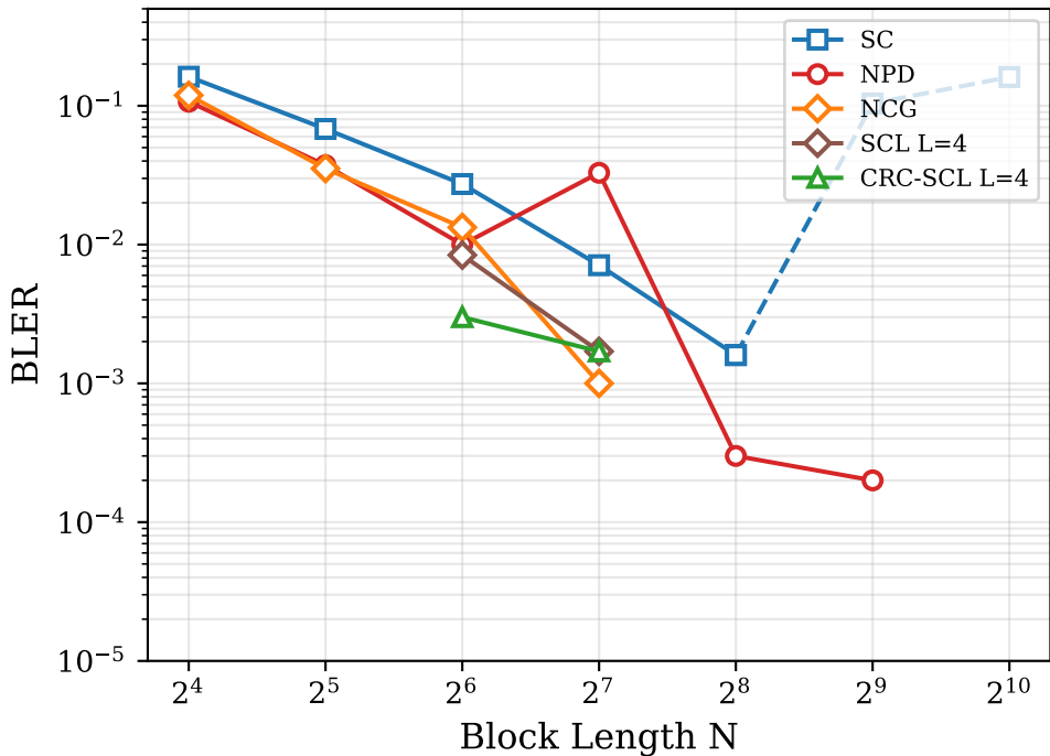
GMAC Class C (6 dB): BLER vs N
