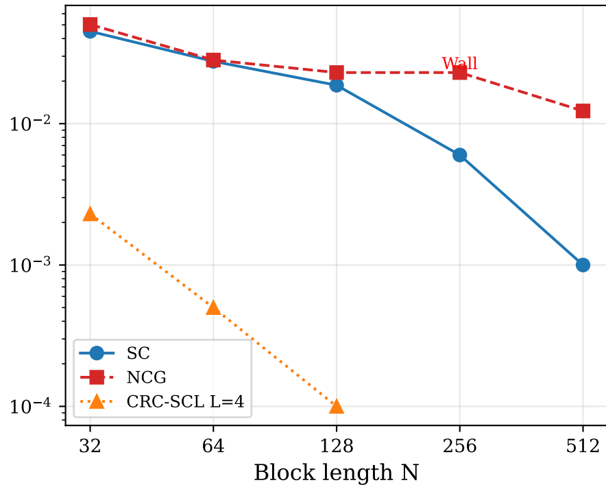
(a) GMAC Class B (SNR=6dB)
