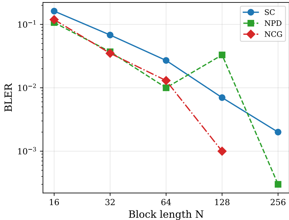
(b) GMAC Class C (SNR=6dB)
