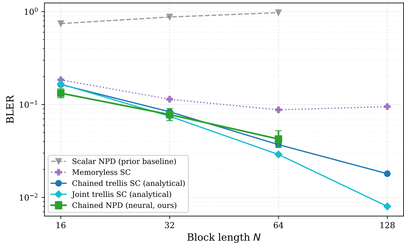
ISI-MAC ( h = 0.3 , SNR = 6 dB): chained NPD vs trellis SC
