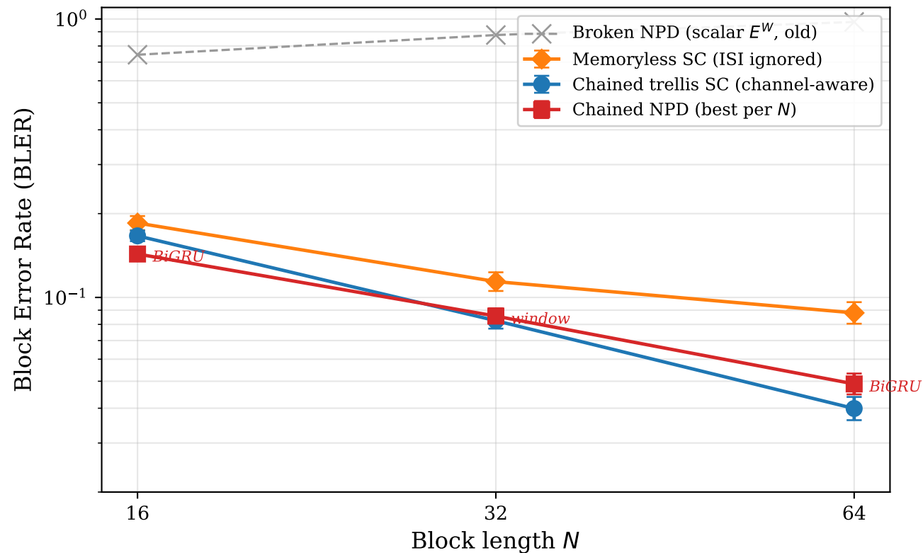
ISI-MAC ( h = 0.3 , SNR = 6 dB, Class C corner rate) Audited 10K-codeword measurements, Wilson 95% CI
