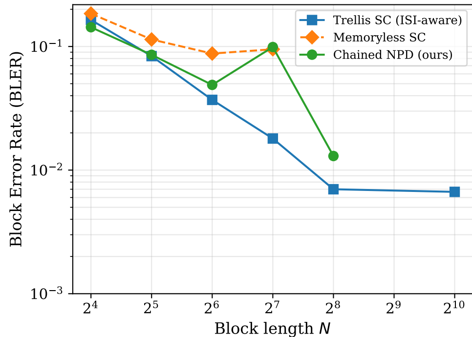
ISI-MAC Class C, SNR = 6 dB, h = 0.3
