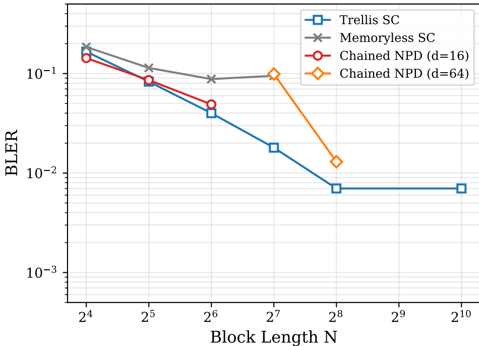
ISI-MAC Class C ( h=0.3 , 6 dB): BLER vs N
