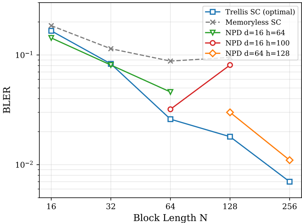
ISI-MAC Class C ( h = 0.3 , SNR = 6 dB): BLER vs N
