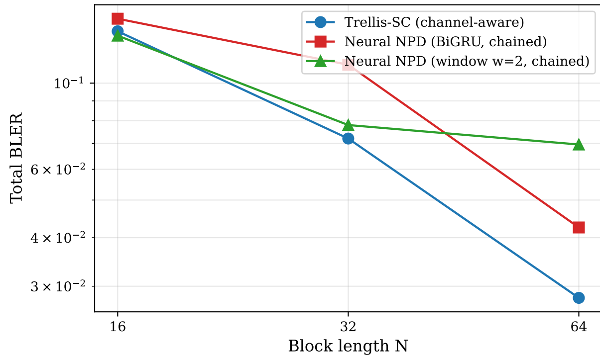
ISI-MAC ( h = 0.3 , SNR=6dB): Chained NPD vs Trellis-SC
