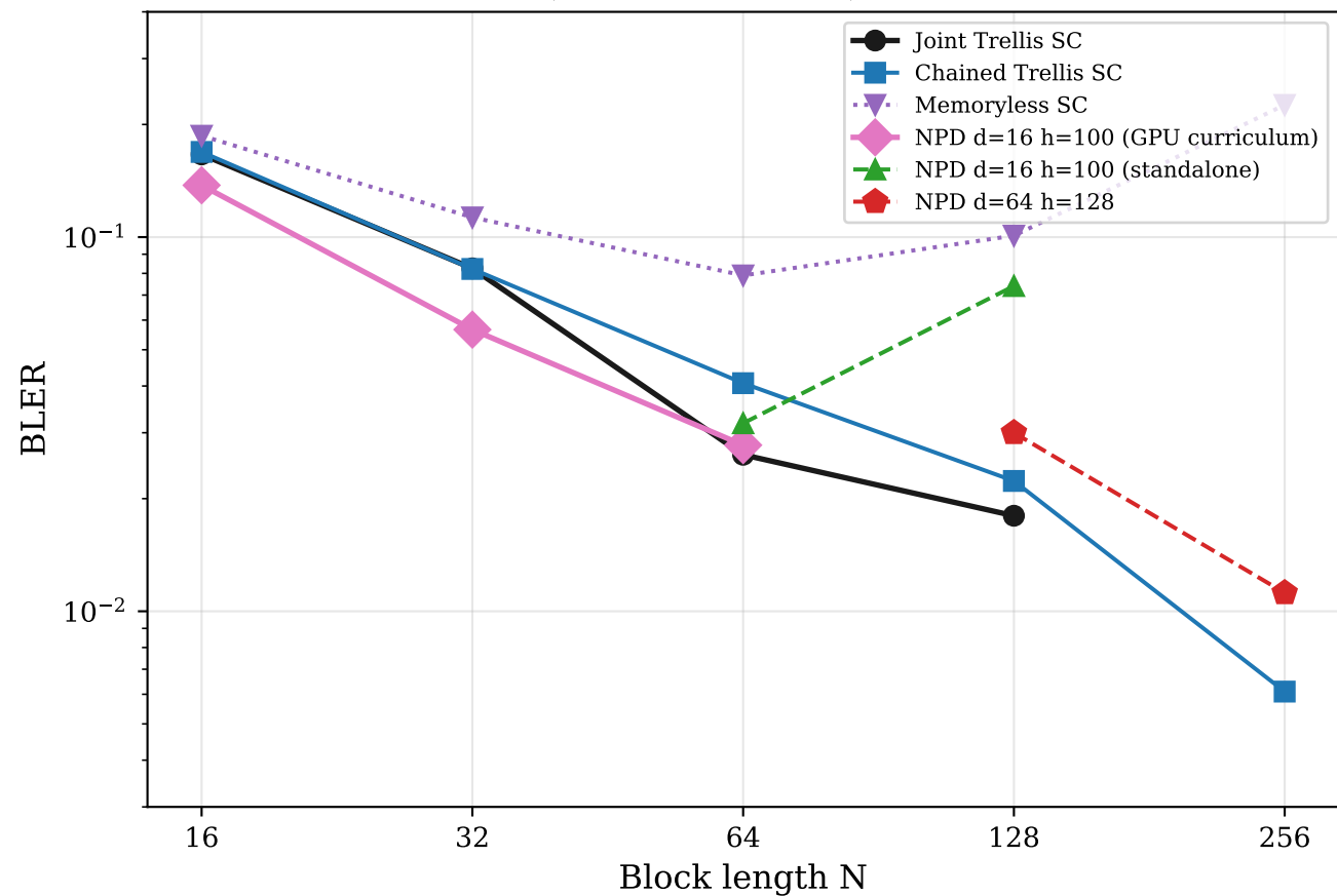
ISI-MAC ( h=0.3 , SNR=6dB): All Decoders
