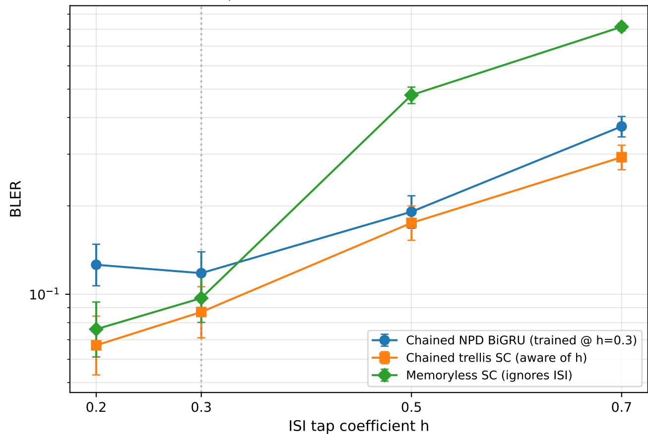
ISI-MAC h-sweep (N=32, SNR=6.0 dB, ku=7, kv=15, 1000 codewords)
