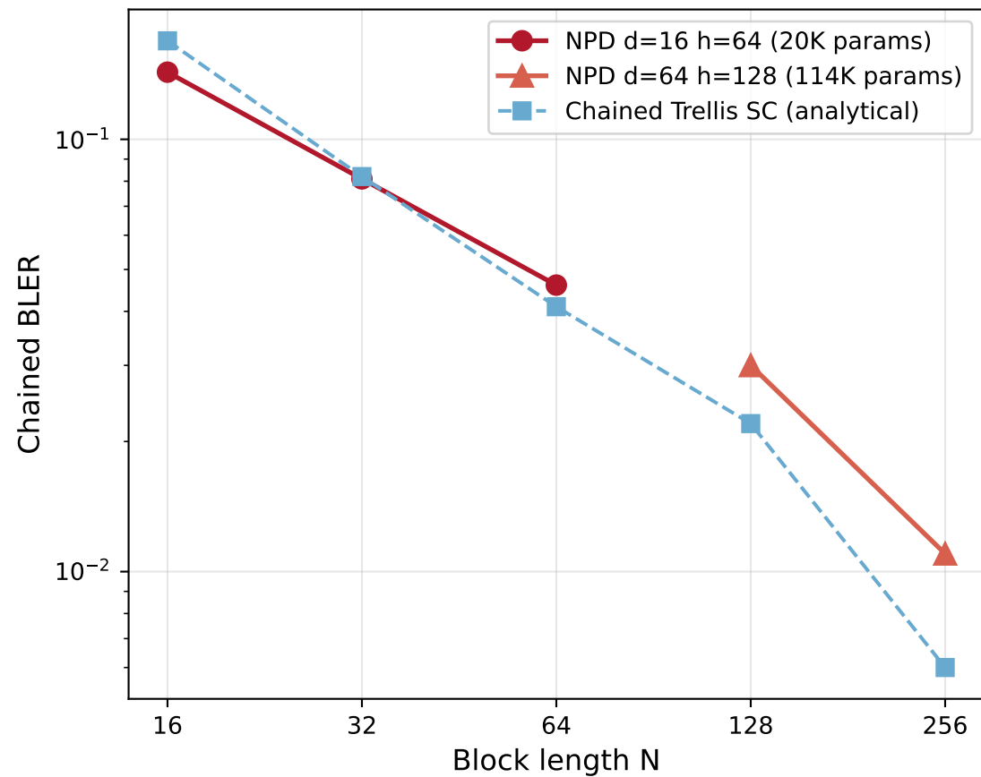
ISI-MAC BLER vs N
