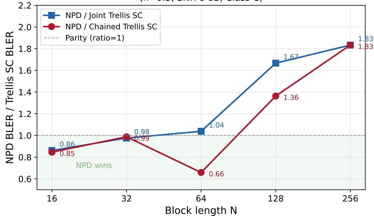
ISI-MAC: Neural decoder gap vs analytical decoder ( h=0.3 , SNR 6 dB, Class C)
