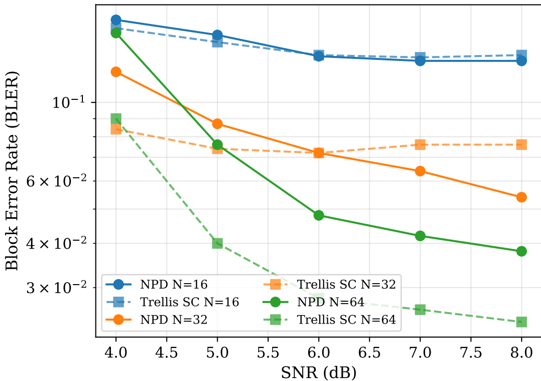
ISI-MAC Class C: SNR sweep, h = 0.3
