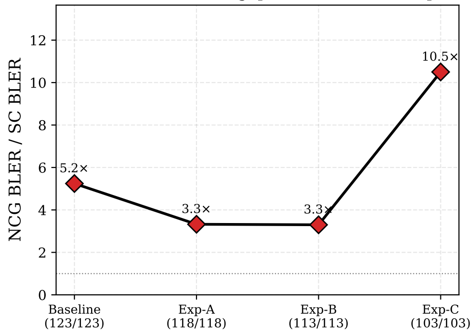
(b) NCG/SC ratio — gap widens as rate drops
