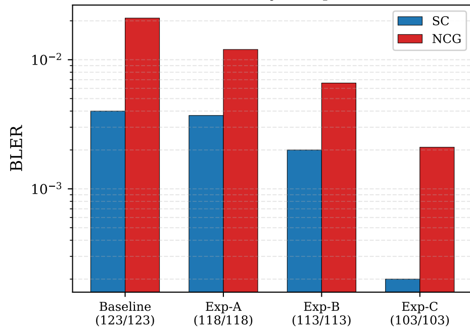
(a) BLER by rate point
