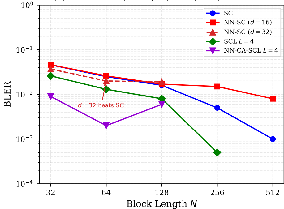
(b) GMAC: Z = (1-2X) + (1-2Y) + W , SNR=6dB
