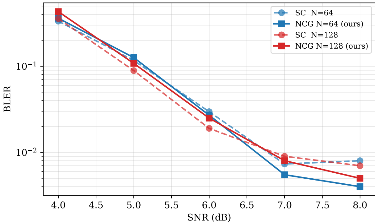
Multi-SNR waterfall — GMAC Class B (6 dB design, no retraining)
