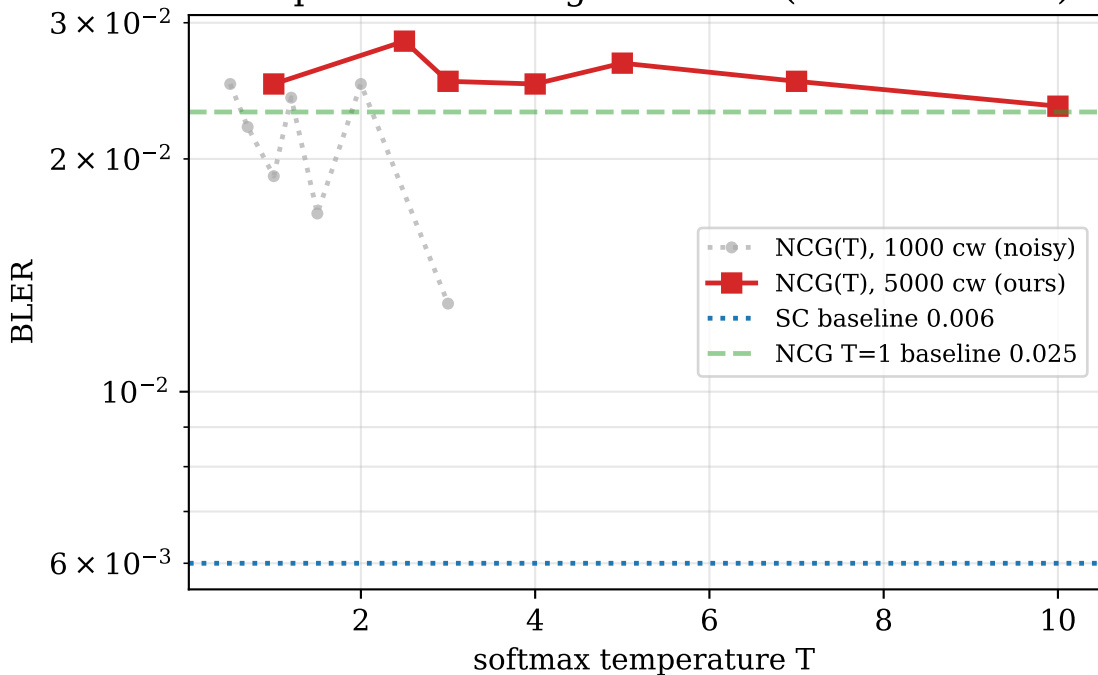
Temperature scaling at N=256 (GMAC Class B)
