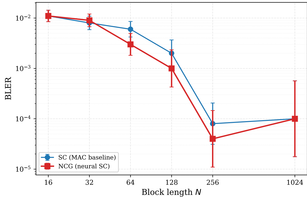
BEMAC Class B: NCG vs SC (sum-rate = 1)
