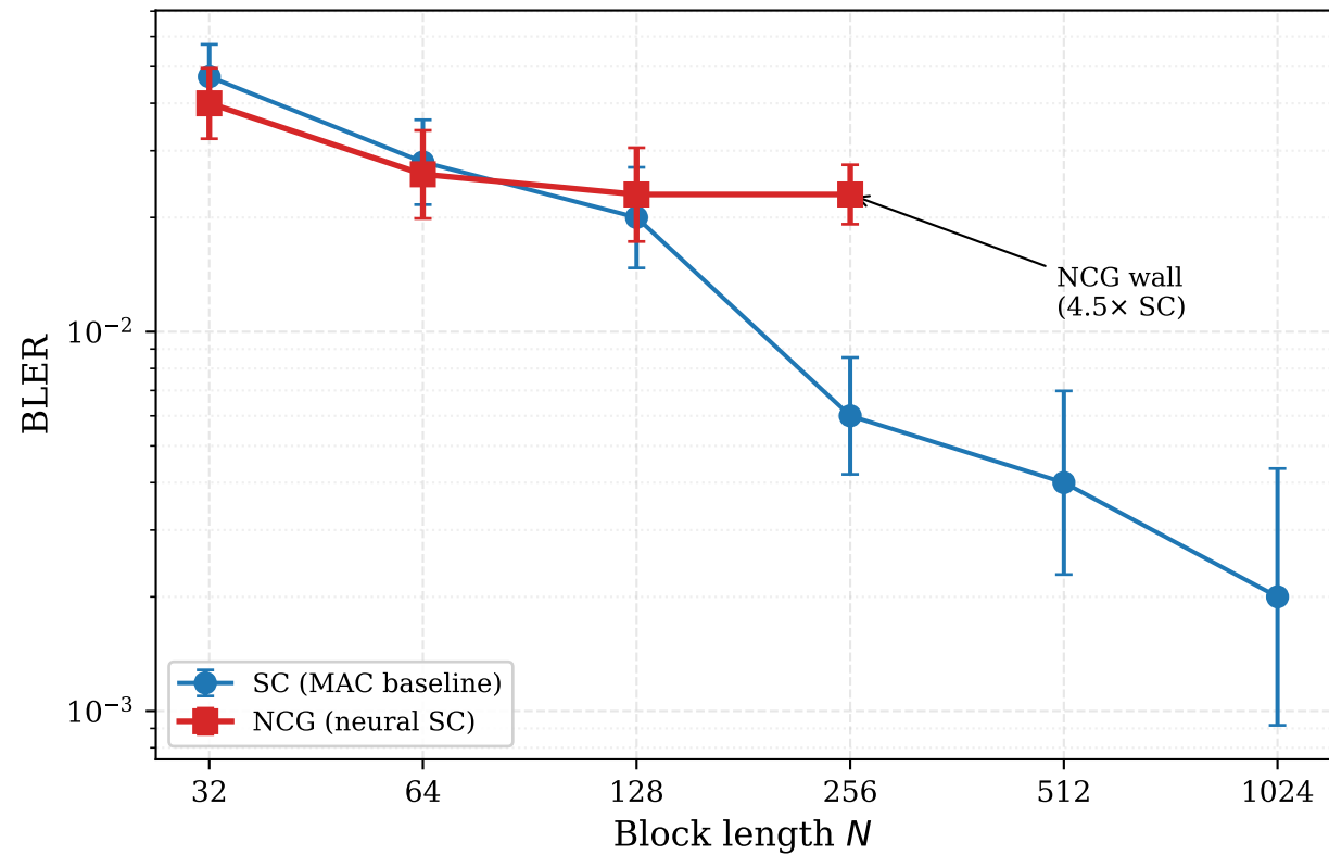
GMAC Class B: NCG vs SC (sum-rate \approx 0.96 , SNR = 6 dB)
