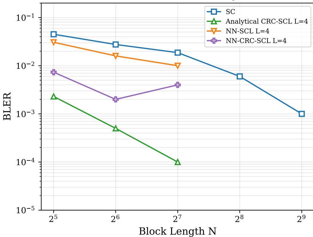
GMAC Class B: NN-SCL vs Analytical SCL
