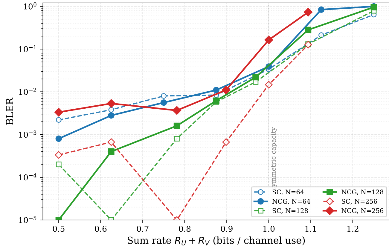
GMAC Class B: rate sweep (NCG solid, SC dashed) — SNR = 6 dB
