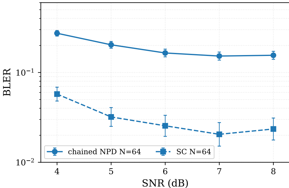
Chained NPD vs analytical SC — GMAC Class C (corner rate)
