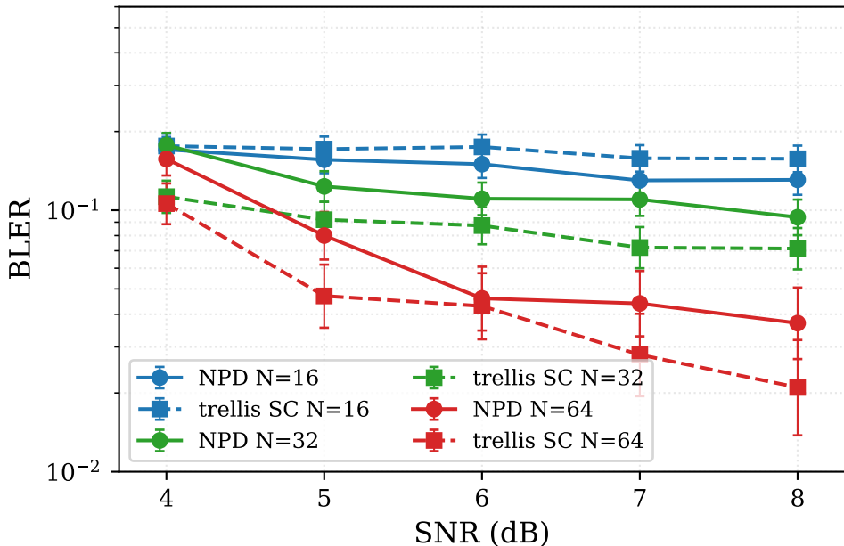
Chained NPD vs chained trellis SC — ISI-MAC ( h = 0.3 )
