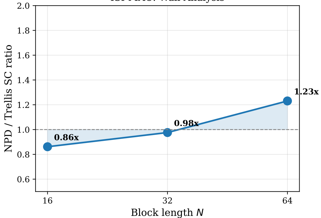
ISI-MAC: Wall Analysis
