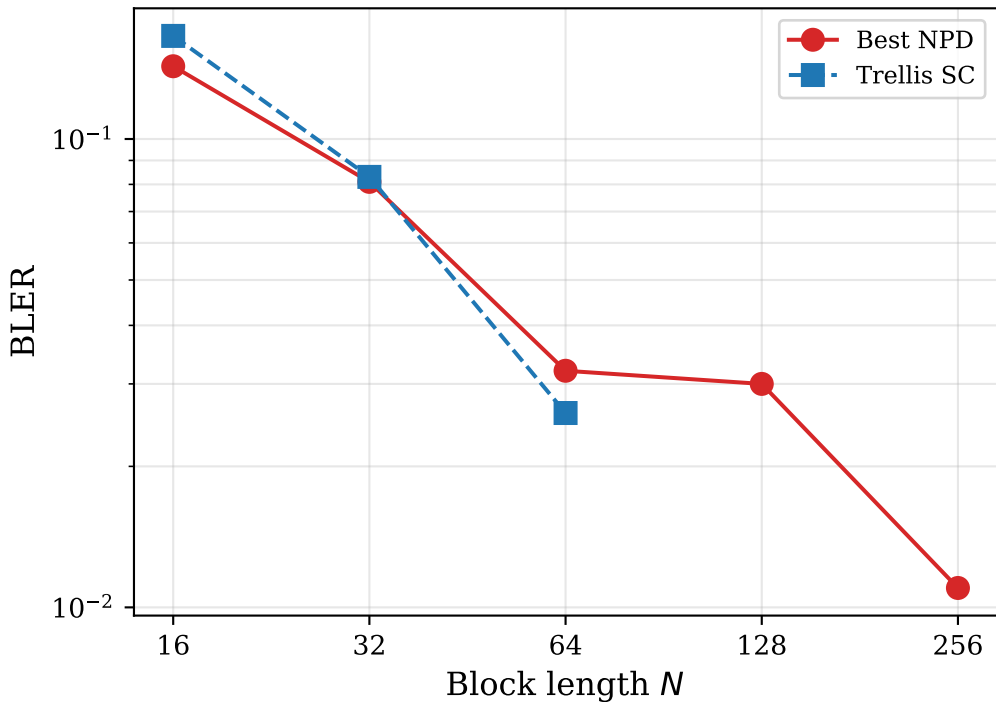
ISI-MAC: BLER vs N
